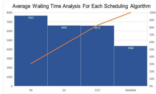
Fig 7: Average Waiting Time Comparison For Improved-Max-Min, FCFS, SJF And RR
