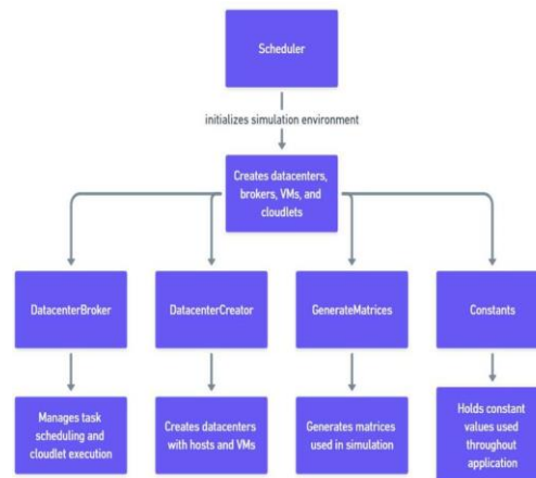
Fig 3: High Level Design For The Algorithm
