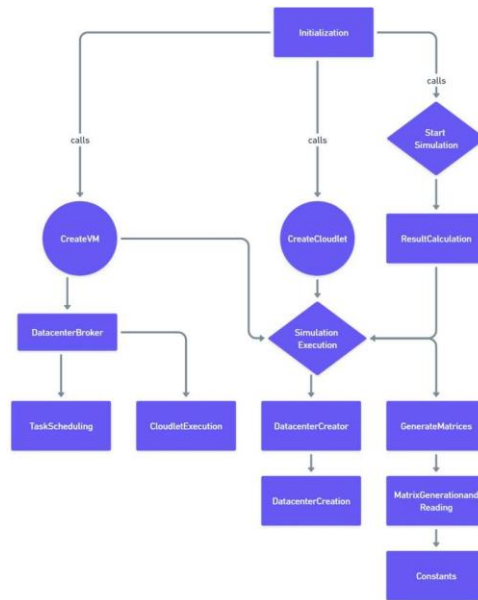
Fig 4: Low Level Design For The Algorithm
