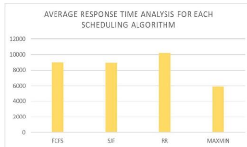
Fig 8: Average Response Time Comparison For Improved-Max-Min, FCFS, SJF And RR
