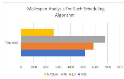
Fig 5: Makespan Comparison For Improved-Max-Min, FCFS, SJF And RR
